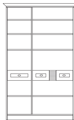
SK02 (1500x2250x400)
